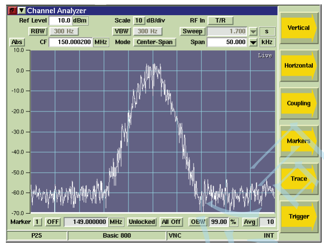
Spectrum Analyzer
